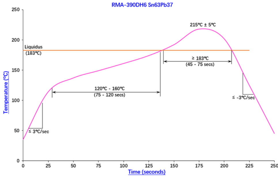
Figure 1: Typical 63Sn37Pb Reflow Profile
