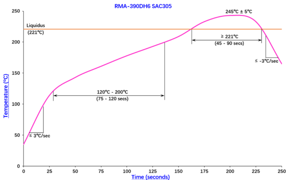
Figure 2: Typical SAC Reflow Profile
